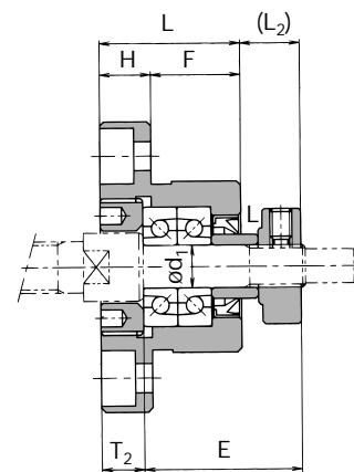
Montagemethode B
