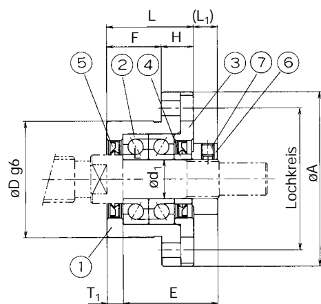
Montagemethode A
