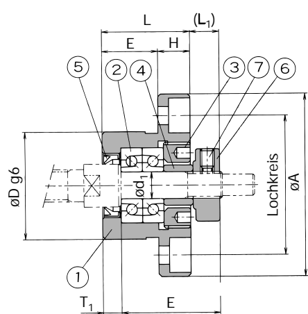
Montagemethode A
